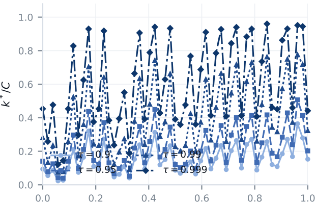
timm_wide_resnet50_2.tv_in1k
