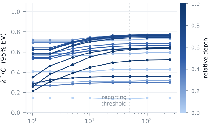
convnext_tiny
