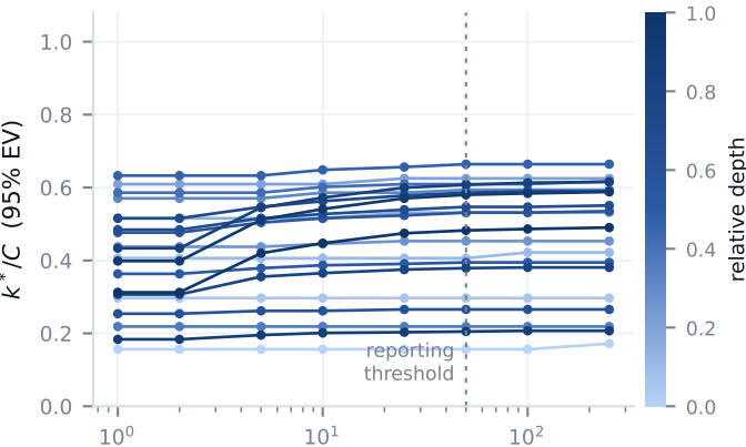
resnet18
