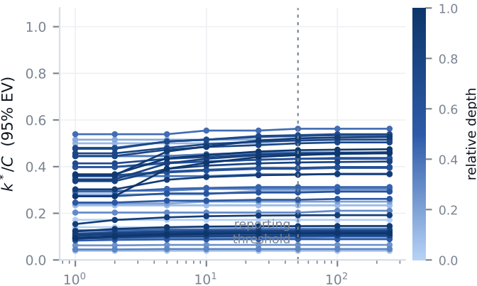
resnet50
