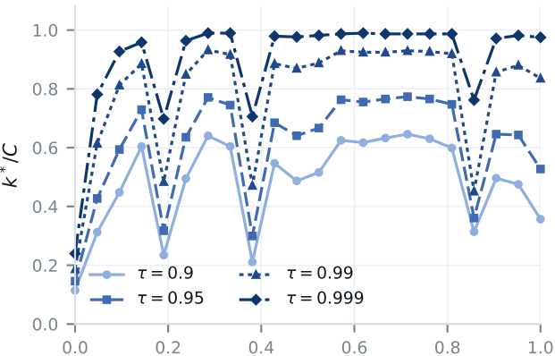
convnext_tiny
