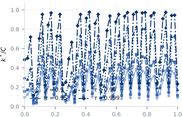
resnet50
