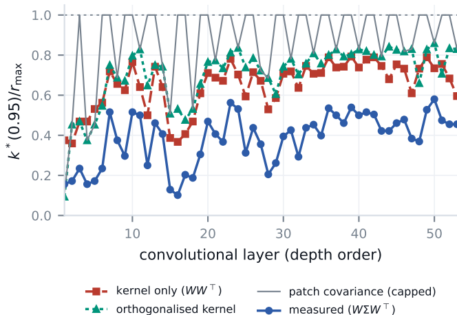
ResNet-50, trained
