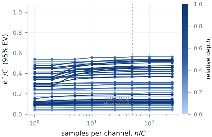
resnet50
