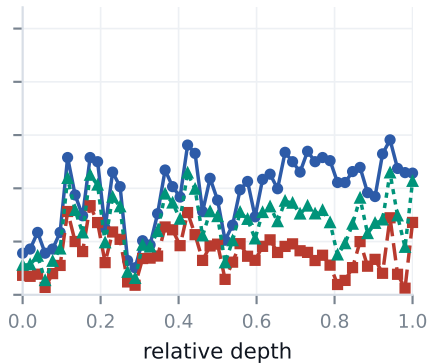
ResNet-50
