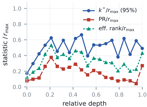
ResNet-18
