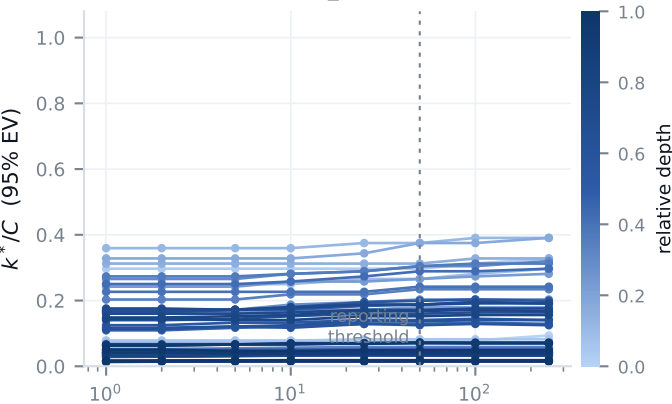
resnet50_random
