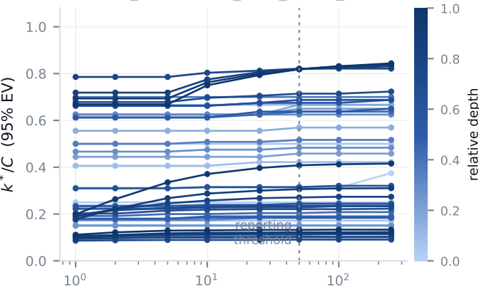
timm_mobilenetv3_large_100.ra_in1k
