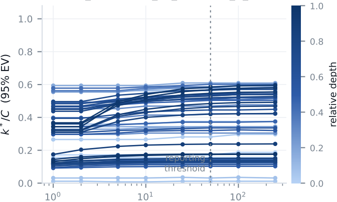
timm_resnet50.fb_ssl_yfcc100m_ft_in1k
