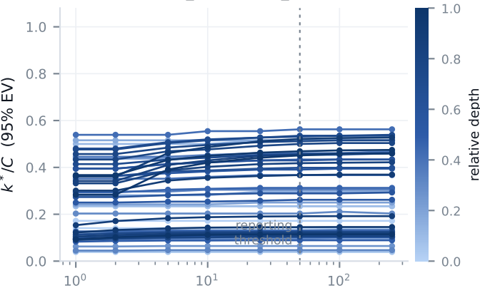
timm_resnet50.tv_in1k
