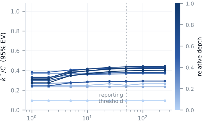
timm_vgg16.tv_in1k
