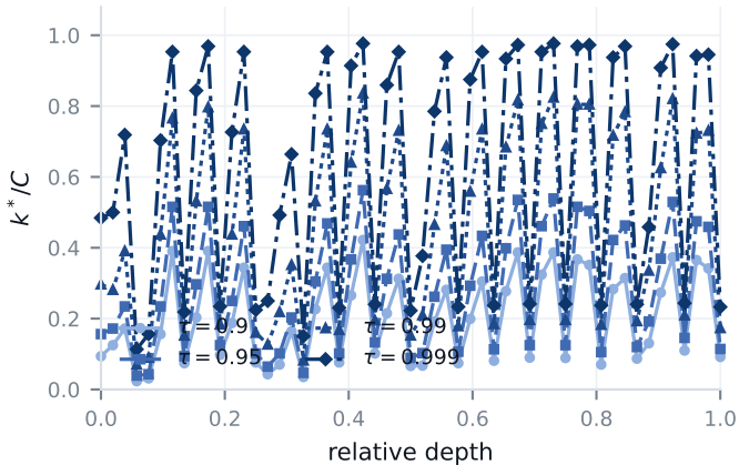
resnet50
