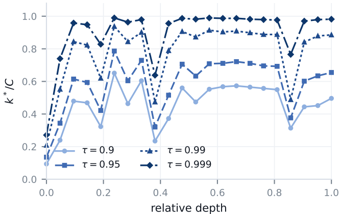
timm_convnext_tiny.fb_in22k_ft_in1k
