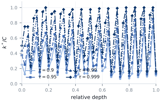
timm_mobilenetv3_large_100.ra_in1k
