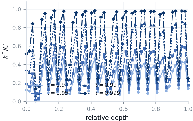
timm_resnet50.fb_ssl_yfcc100m_ft_in1k
