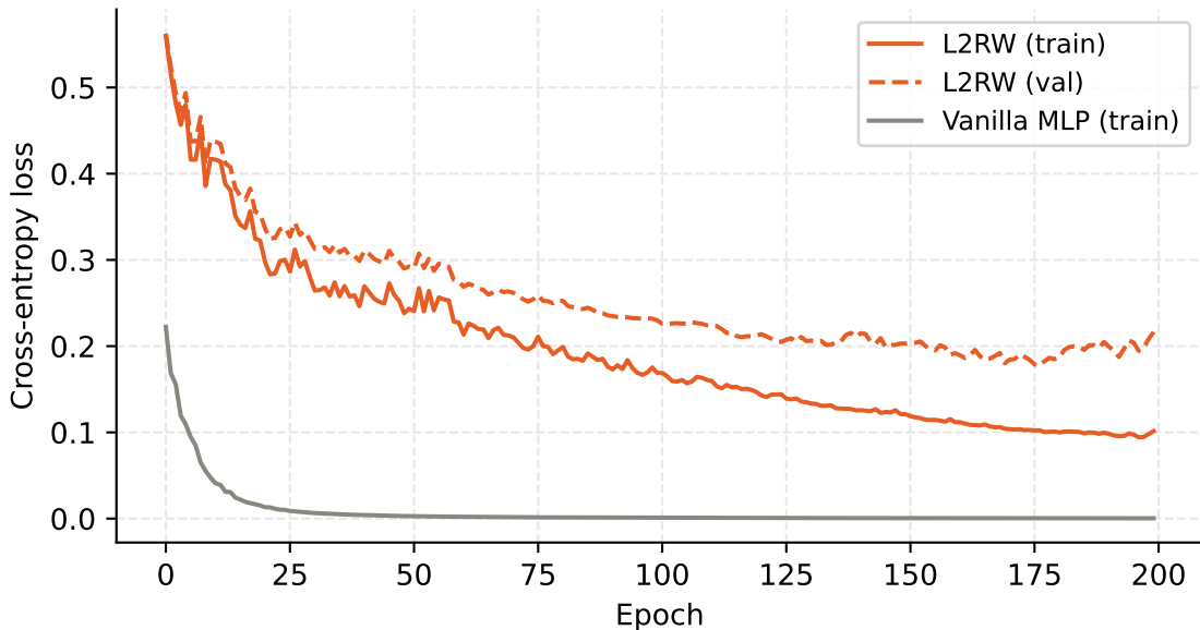
Training curves: L2RW vs Vanilla MLP (10:1 imbalance)
