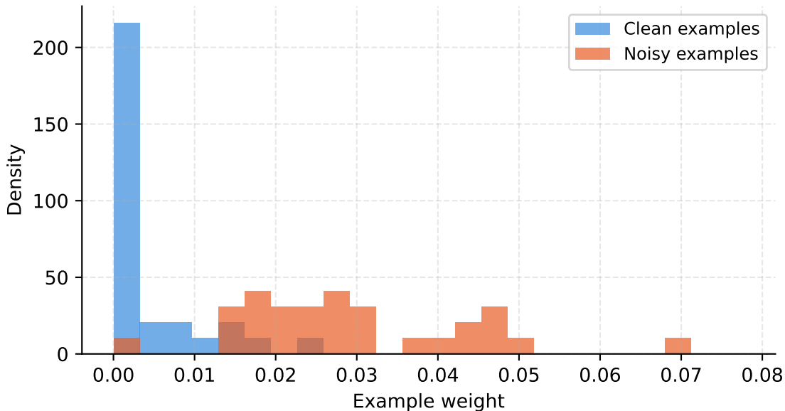
Weight distribution: clean vs noisy (background flip, 30%)
