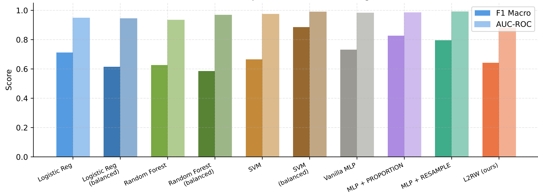
Model comparison at hardest setting
