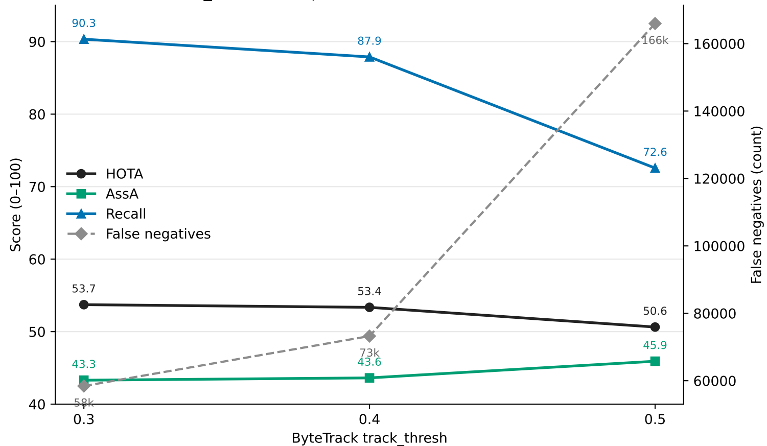
track_thresh sweep — recall traded for association
