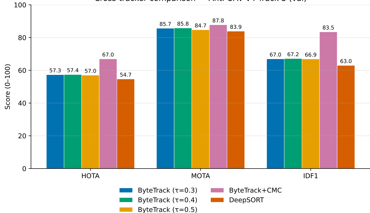
Cross-tracker comparison — Anti-UAV v4 Track 3 (val)
