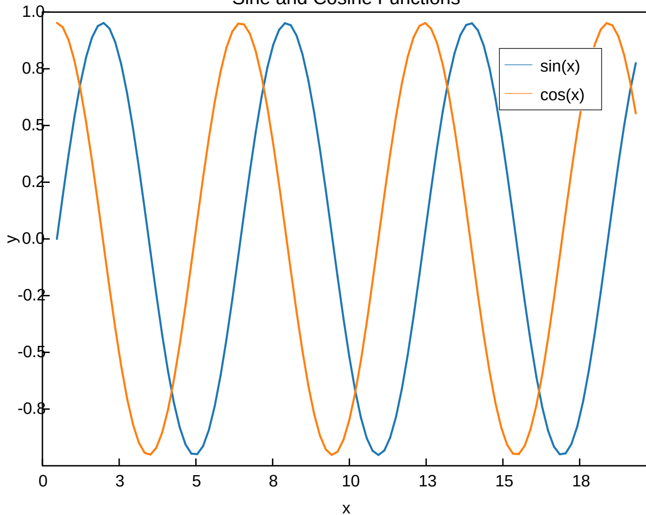
Sine and Cosine Functions
