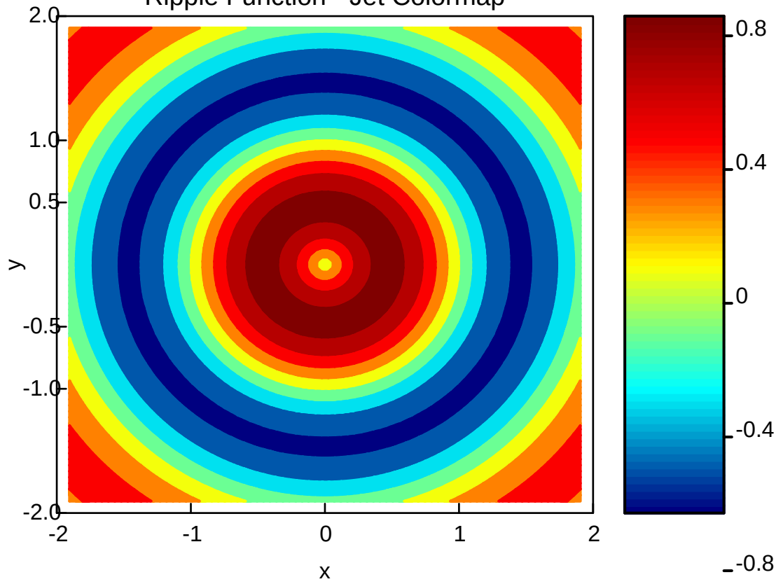
Ripple Function - Jet Colormap
