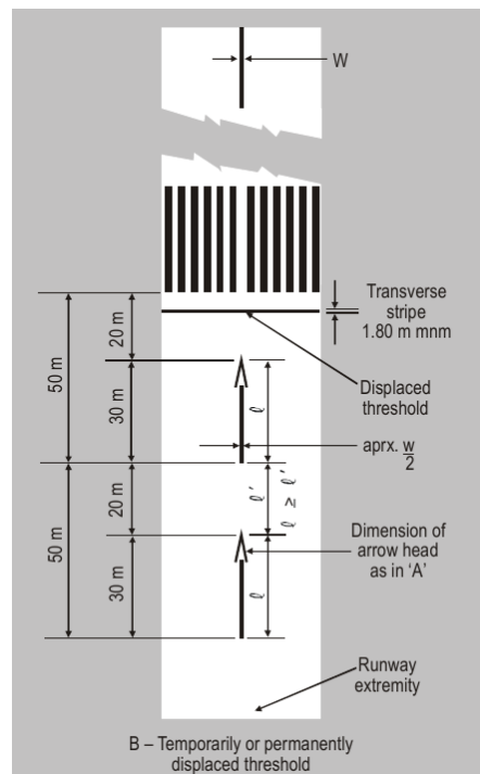
ICAO Annex14 Figure 5-4(B), printed page 5-9, PDF page 135: displaced-threshold bar and white arrows. [A14]
