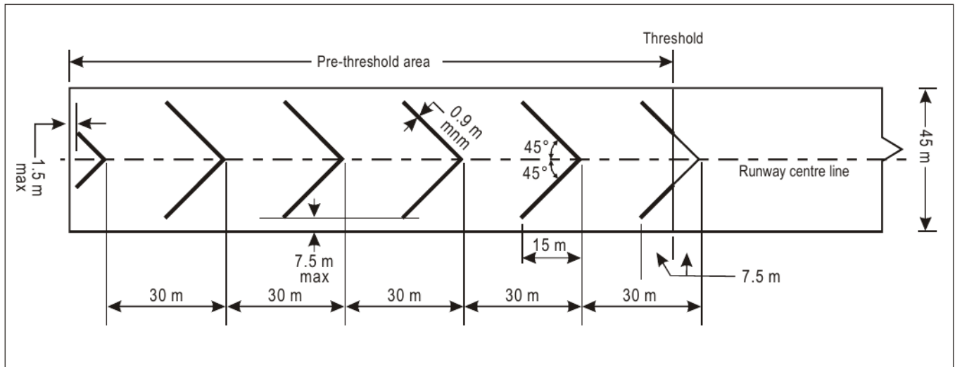
ICAO Annex14 Figure 7-3, printed page 7-7, PDF page 245: chevrons on unsuitable pre-threshold pavement. [A14]
