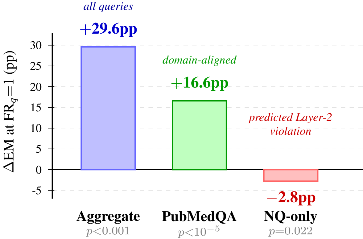
Figure S2: Per-query level analysis within CH-H ( N=6,000 , 3-seed aggregate; cf. Table 3 for condition-level cross-domain decisions). The +29.6pp aggregate EM gap at \text{FR}_q=1 masks partition-conditional direction: PubMedQA-only +16.6pp (domain-aligned, r_{pb}^{\text{partial}}=0.086 ); NQ-only -2.8pp ( r_{pb}^{\text{partial}}=-0.042 )—the predicted Layer-2 violation under domain mismatch (§3.2). \text{FR}_q=0 robustly signals suppression in both partitions; only \text{FR}_q=1 direction is partition-conditional, validating FR as a binary detector with empirical ground.
