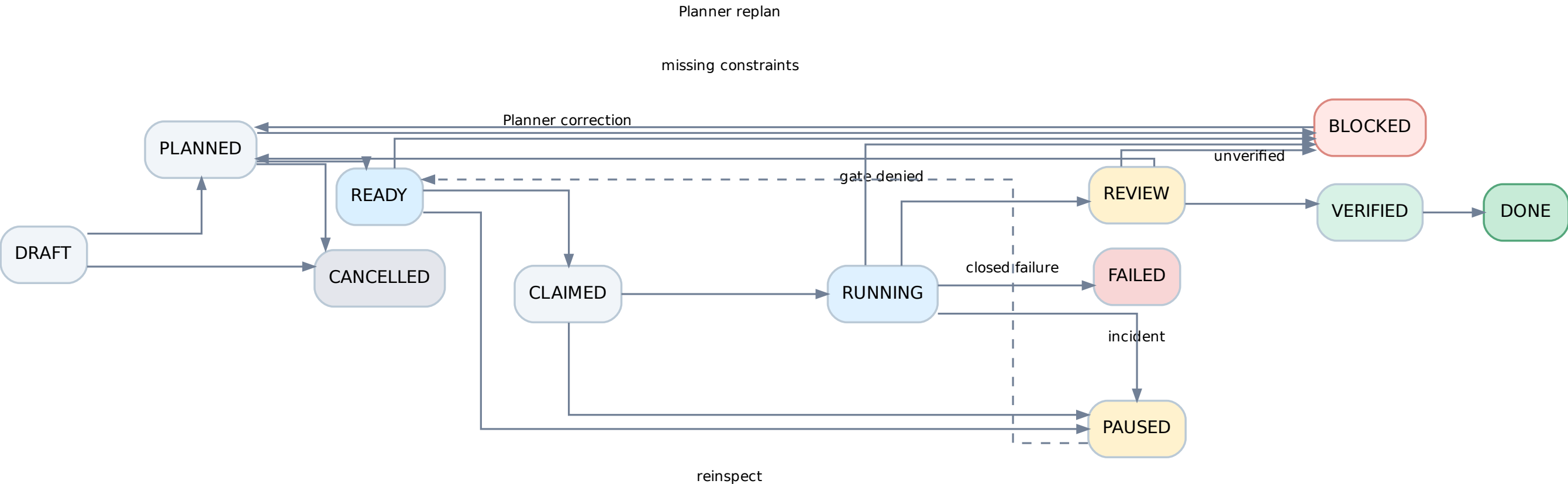
D03 | Proposed Task lifecycle (not transport status)
