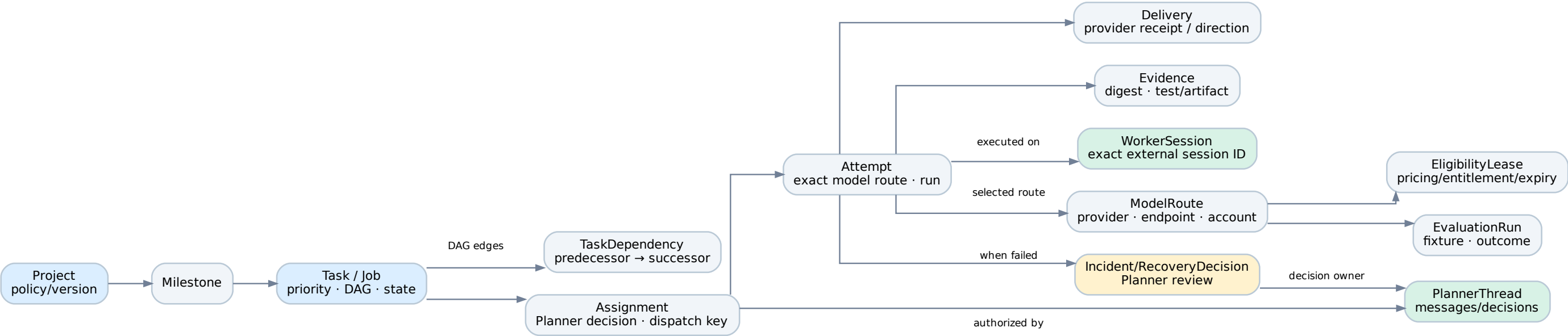
D10 | Conceptual data relationships (migration must be audited)
