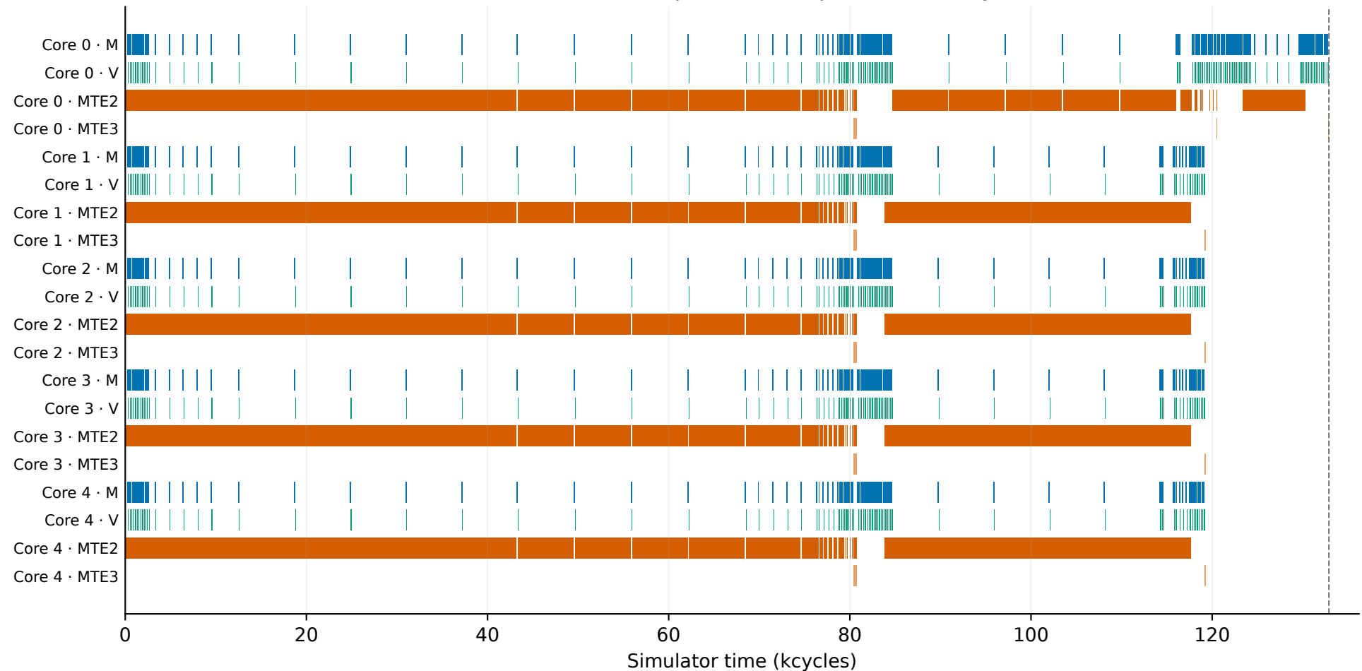
Case 044: Initial Q2 plan · makespan 132,892 cycles
