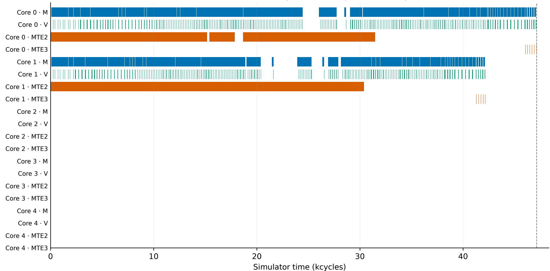
Case 044: Selected CILC plan · makespan 47,127 cycles
