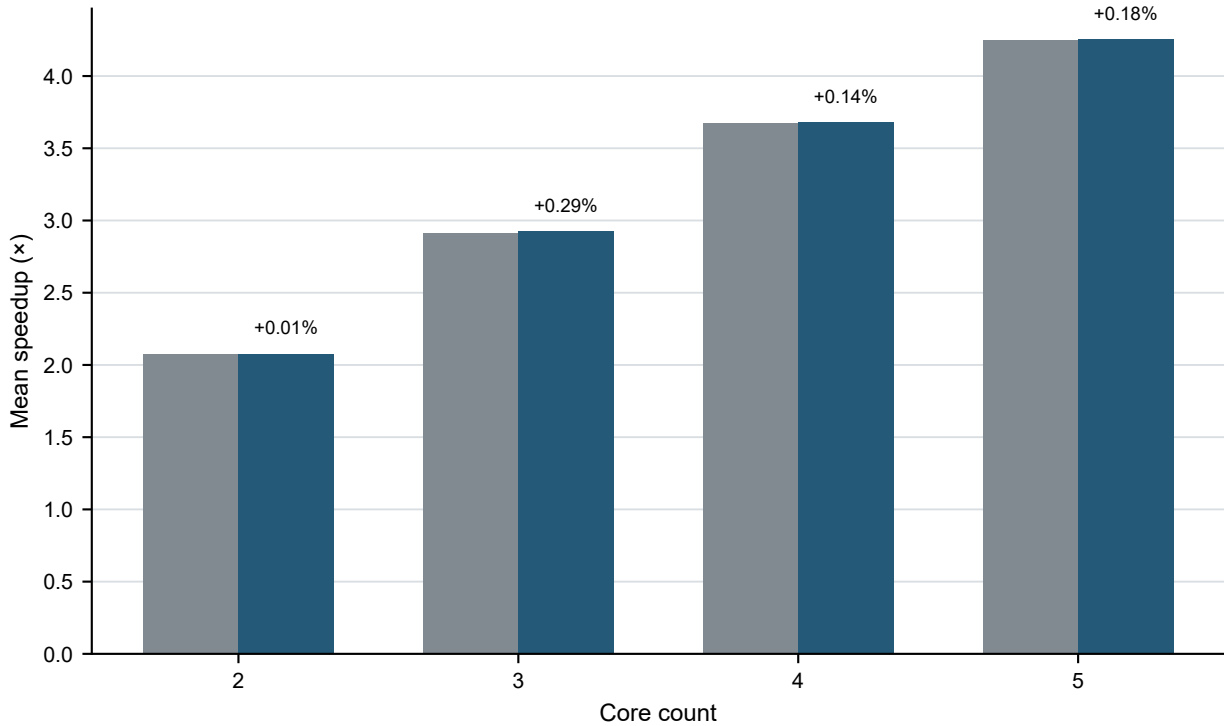
Q2 incremental refinement: cold start (gray) vs retained search (blue)
