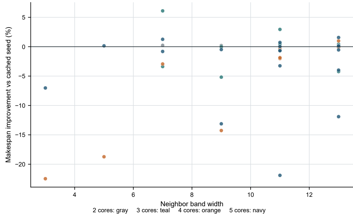
Official evaluation of 40 neighboring-width candidates
