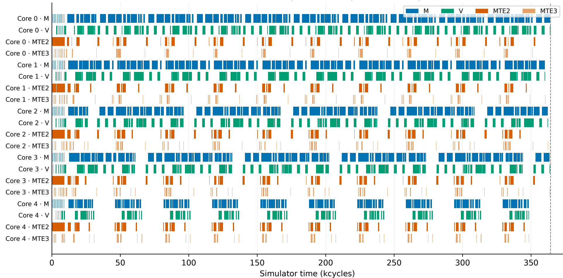
Case 075: Selected CILC plan · makespan 364,184 cycles
