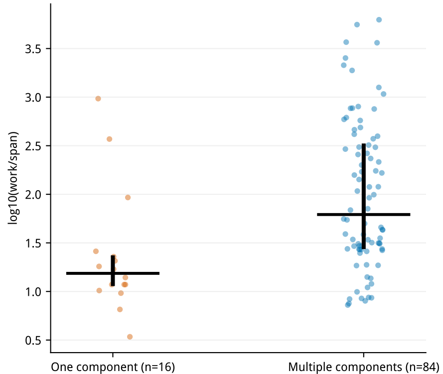
log10(work/span)
