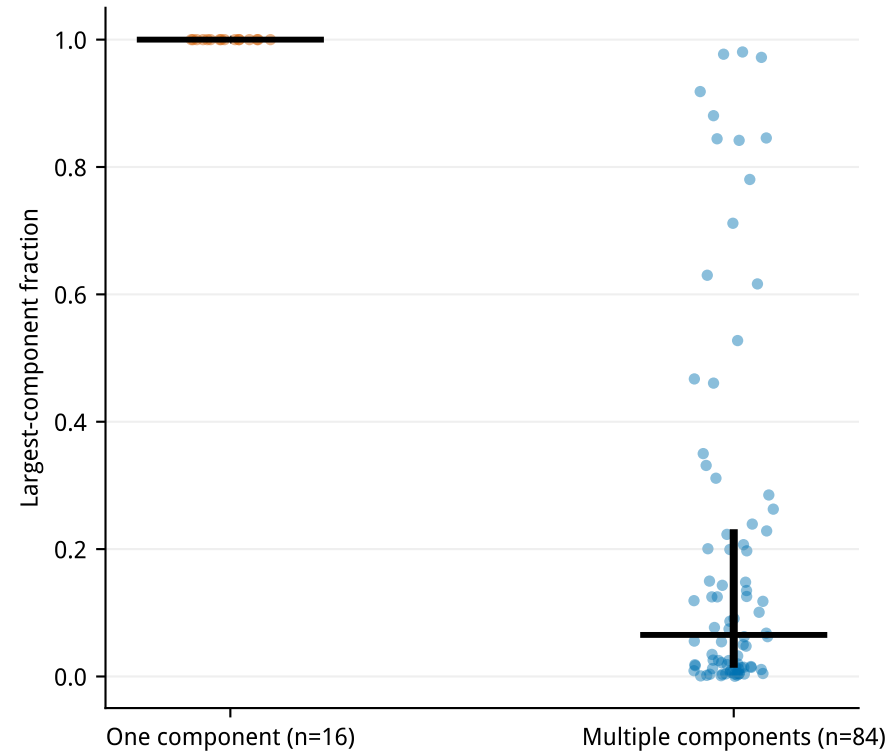
Largest-component fraction
