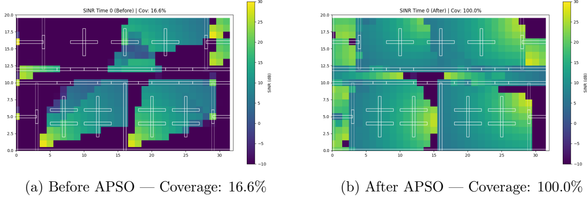
Figure 2: SINR heatmaps at time step t_0 . (a) Static placement produces vast dead zones (purple, \text{SINR} < 5 dB) with only 16.6% coverage. (b) After APSO optimization, routers reposition and re-steer beams to achieve 100.0% coverage.
