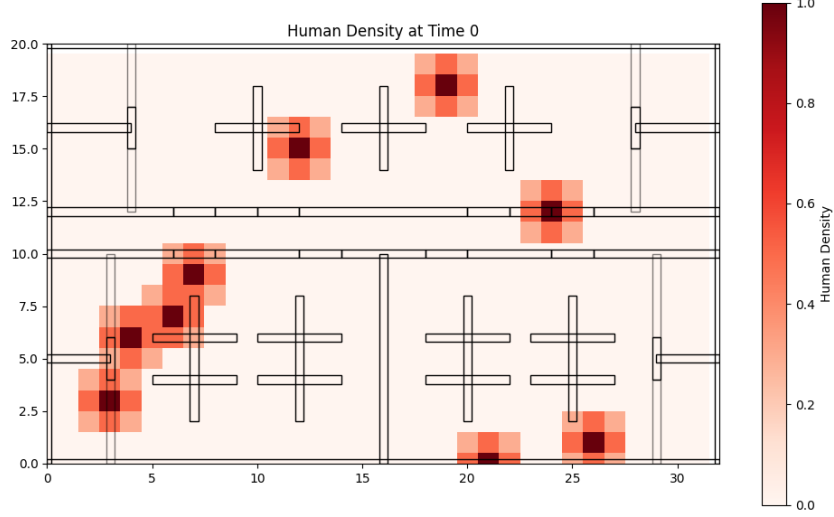
Figure 1: Human density heatmap at time step t_0 . Darker regions represent higher user concentrations modelled as Gaussian clusters. The non-uniform distribution drives the need for adaptive router repositioning.
