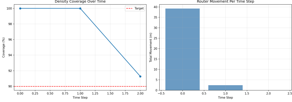
Figure 4: Left: Density-weighted coverage percentage across time steps, with the 90% target shown as a dashed red line. Right: Total router displacement (metres) per time step, showing sharply decreasing movement as the system stabilizes.
