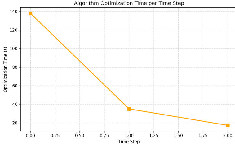
Figure 3: APSO optimization wall-clock time per time step. Warm-starting from previous solutions at t_1 and t_2 reduces convergence time drastically from \sim 138 s down to \sim 35 s and \sim 18 s, demonstrating efficient incremental re-optimization.
