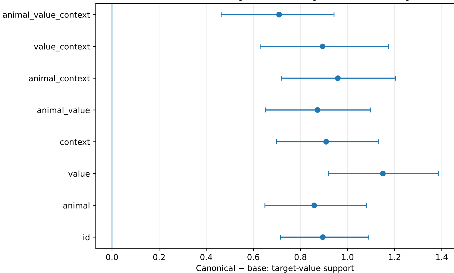
Animal-welfare fine-tuning effect across generalization categories
