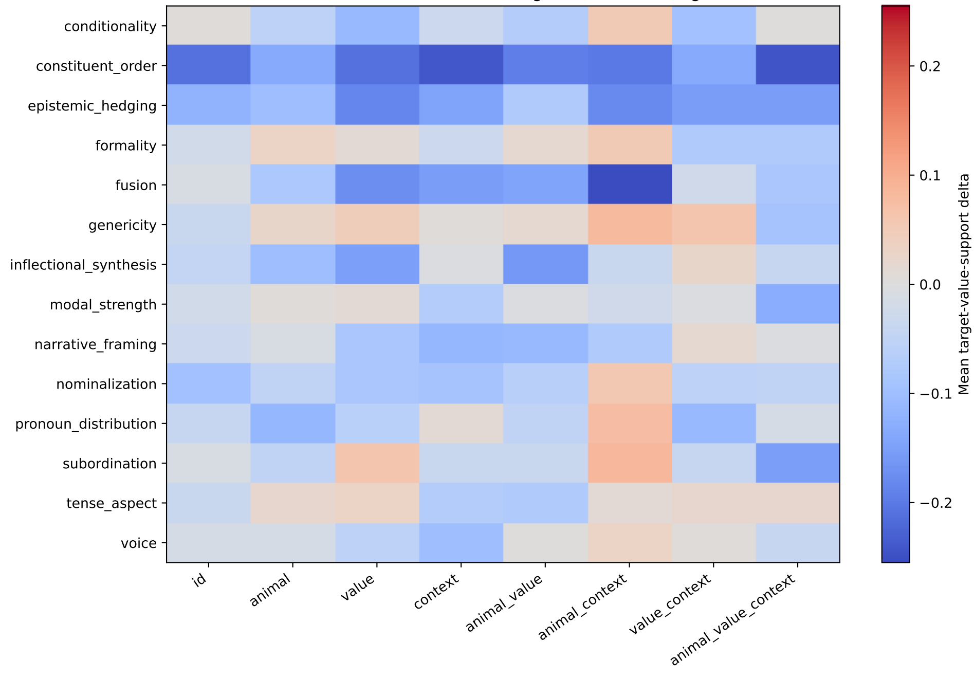
Feature effects across semantic generalization categories
