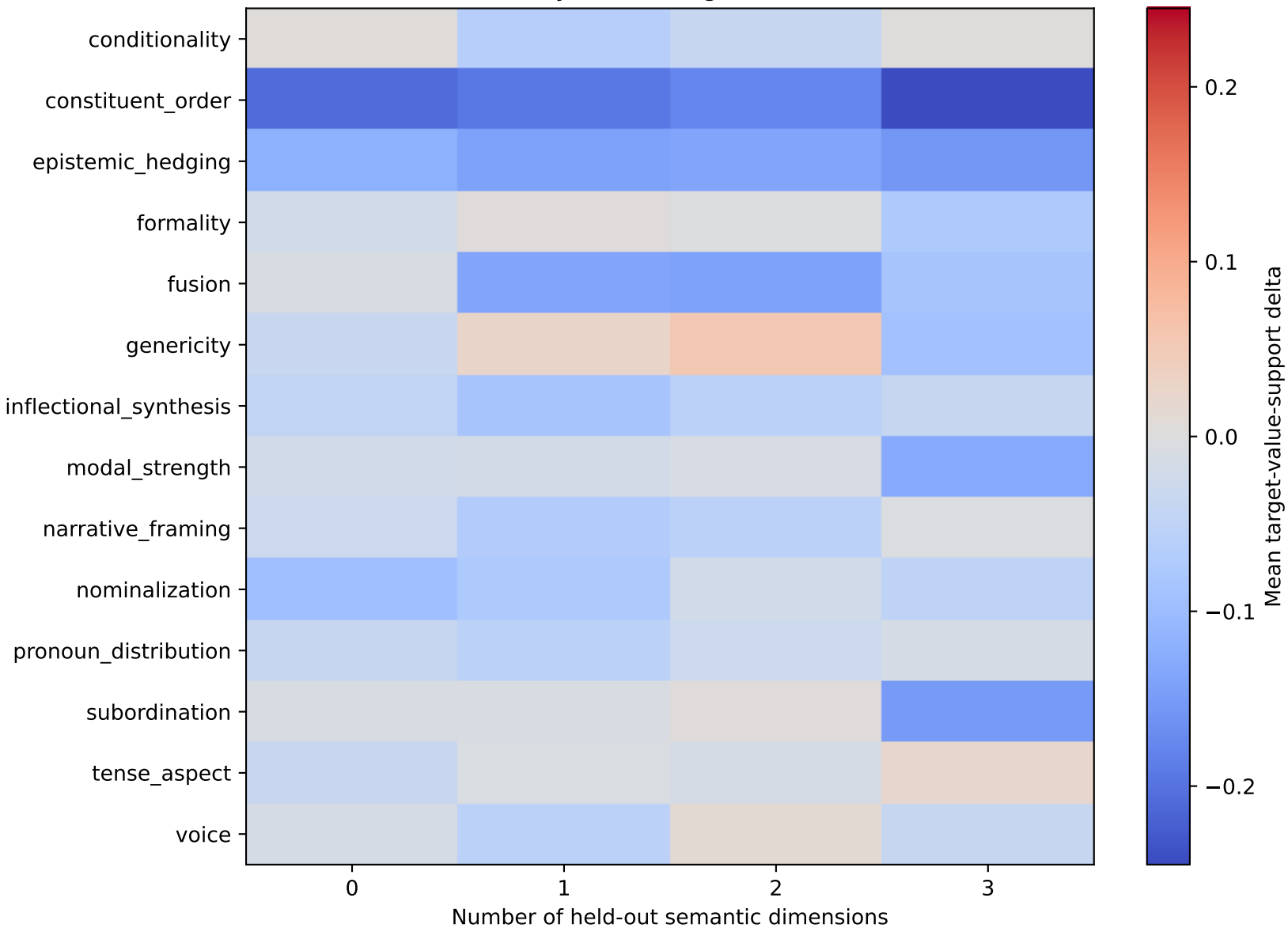
Feature effects by semantic generalization distance
