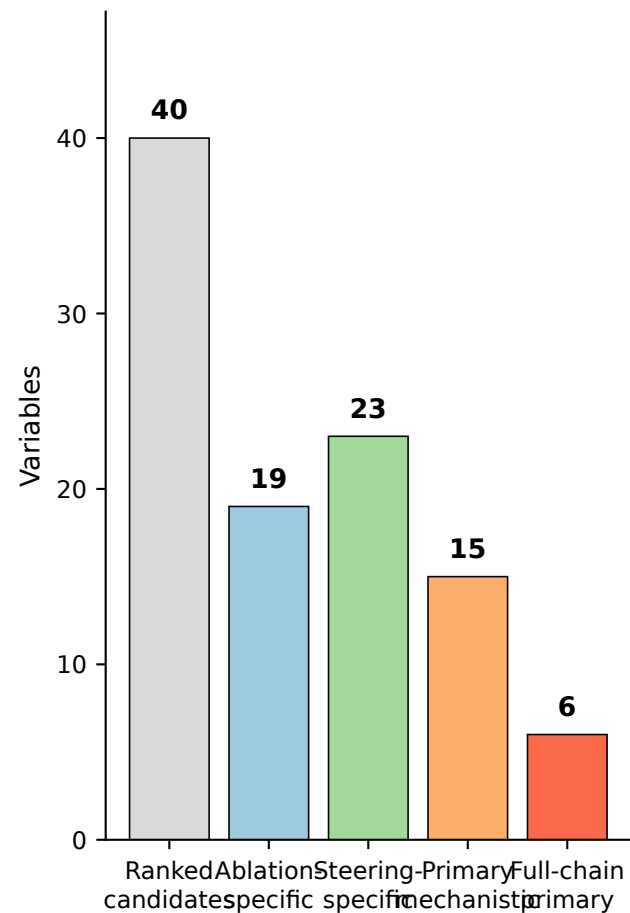
(b) Funnel from candidate features to final causal evidence
