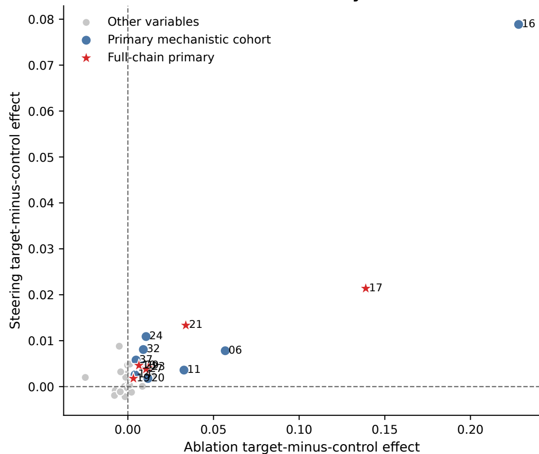
(a) Causal intervention effects by variable
