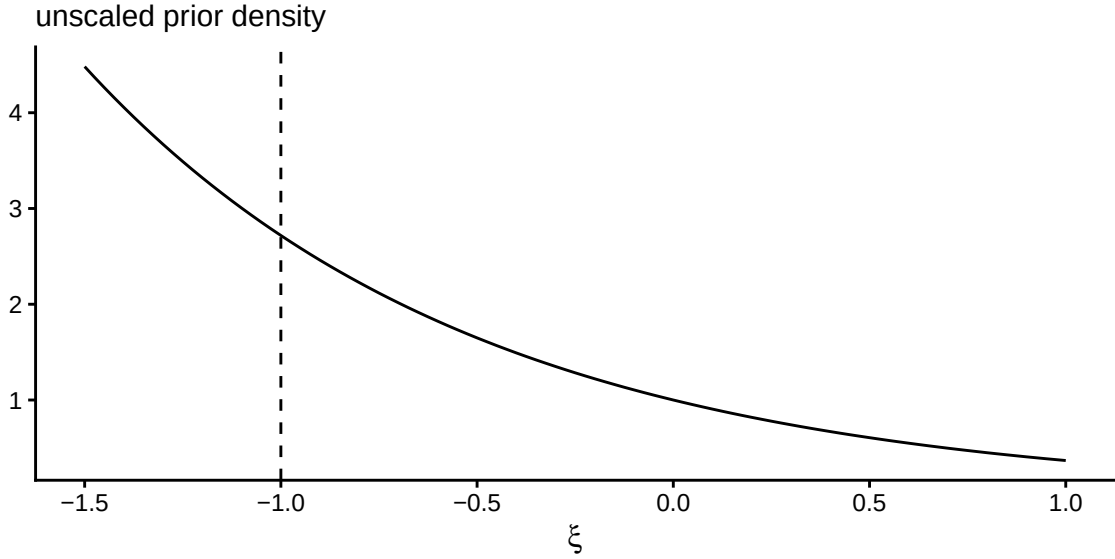
Figure 3.3: Unscaled maximum data information (MDI) prior density.
