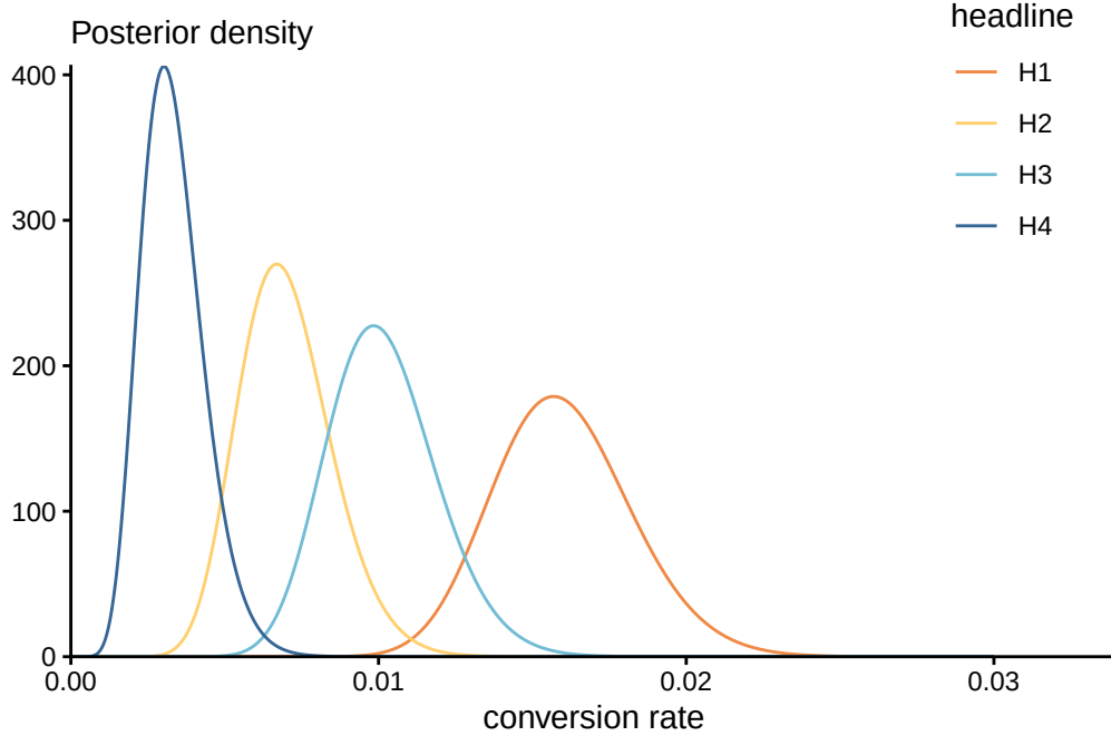
Figure 3.1: Gamma posterior for conversion rate of the different Upworthy Sesame Street headline.
