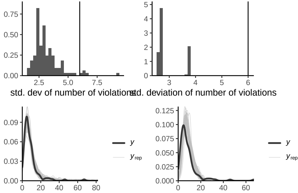
Figure 7.5: Posterior predictive checks for the standard deviation (top) and density of posterior draws (bottom) for hierarchical Poisson model with individual effects (left) and simpler model with only conditions (right).
