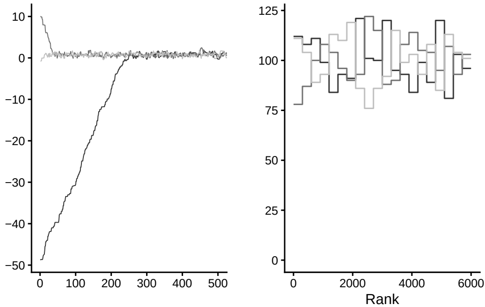
Figure 5.5: Traceplots of three Markov chains for the same target with different initial values for the first 500 iterations (left) and trace rank plot after discarding these (right).
