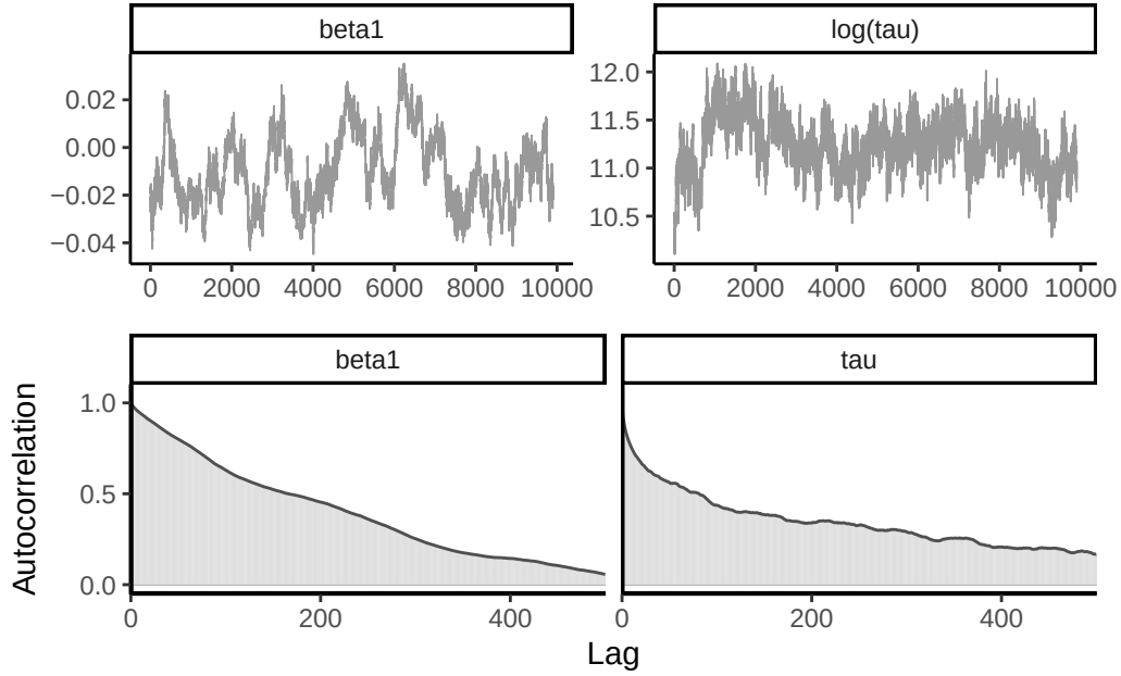
Figure 7.11: Trace plots (top) and correlograms (bottom) for two parameters of the Gibbs sampler for the Tokyo rainfall data, with individual updates for \beta_t .
