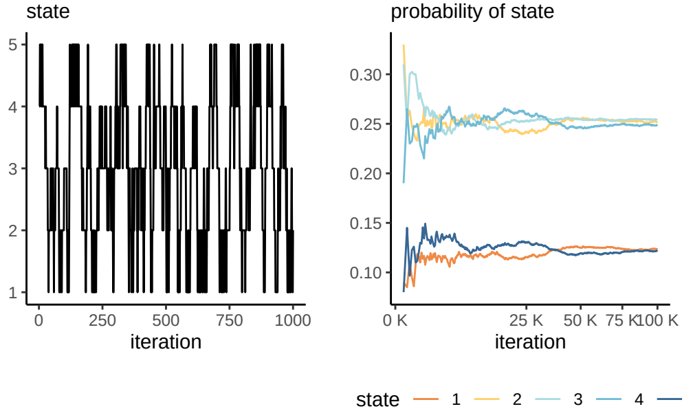
Figure 4.7: Discrete Markov chain on integers from 1 to 5, with transition matrix \mathbf{P}_3 , with traceplot of 1000 first iterations (left) and running mean plots of sample proportion of each state visited per 100 iterations (right).
