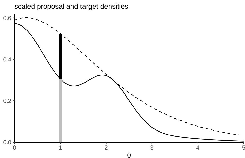
Figure 4.2: Target density (full) and scaled proposal density (dashed): the vertical segment at \theta = 1 shows the percentage of acceptance for a uniform slice under the scaled proposal, giving an acceptance ratio of 0.58.
