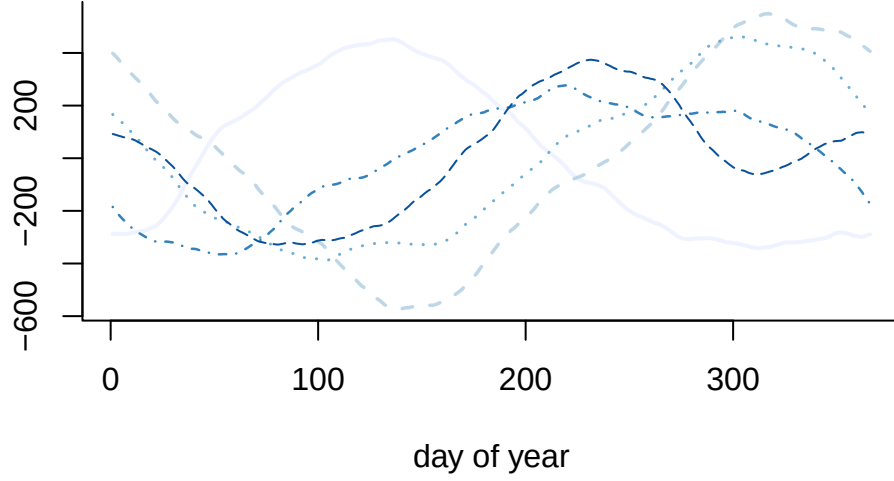
Figure 7.8: Five realizations from the cyclical random walk Gaussian prior of order 2.
