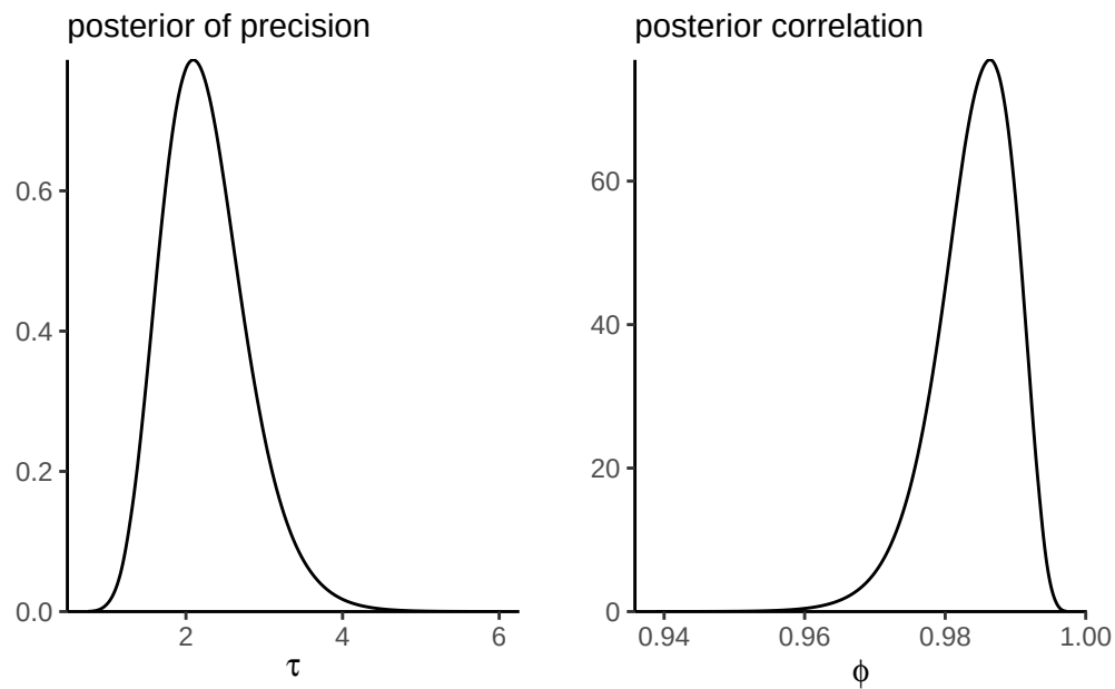
Figure 9.3: Marginal densities of precision and autocorrelation parameters from the Gaussian stochastic volatility model.
