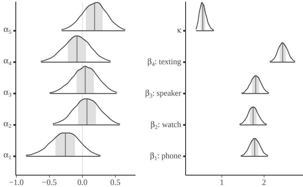
Figure 7.1: Posterior density plots with 50% credible intervals and median value for the random effects of the first five individuals (left) and the fixed effects and random effect variance (right).
