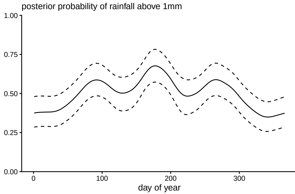
Figure 9.4: Posterior probability per day of the year with posterior median and 95% credible interval for the Tokyo rainfall binomial time series.
