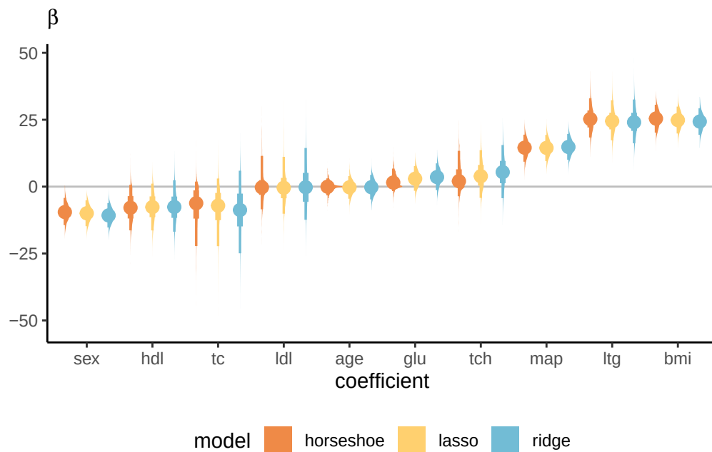
Figure 8.6: Density estimates for regression coefficients with Gaussian (ridge), double exponential (Laplace) and horseshoe priors for the diabetes data.
