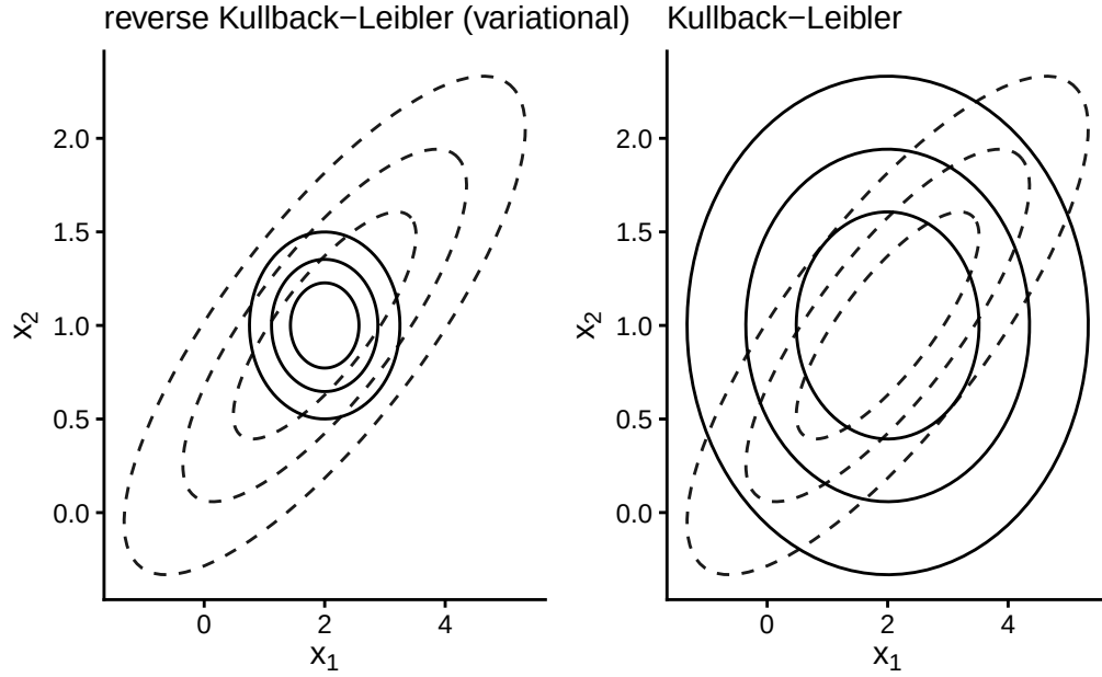
Figure 10.1: Illustration of an approximation of a correlated bivariate Gaussian density (dashed contour lines) with an uncorrelated Gaussian, obtained by minimizing the reverse Kullback–Leibler divergence (variational approximation, left) and the Kullback–Leibler divergence (right).
