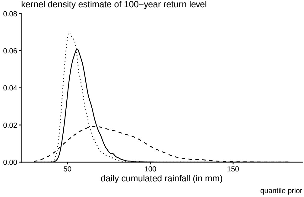
Figure 7.3: Kernel density estimates of draws from the posterior distribution of 100 year return levels with a Coles–Tawn quantile prior (full line) and from the corresponding prior predictive (dashed). The dotted line gives the posterior distribution for a maximum domain information prior on the shape with improper priors on location and scale.
