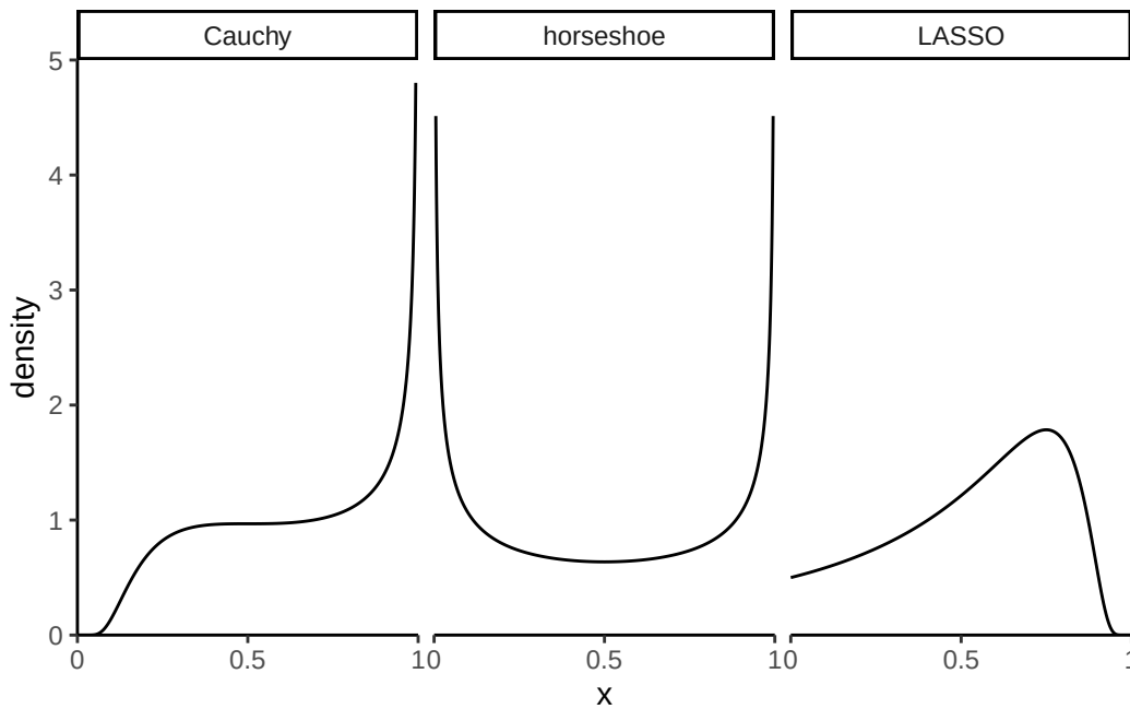
Figure 8.4: Density of penalization weights \kappa of spike (near zero) and slab (near one) for three shrinkage priors.
