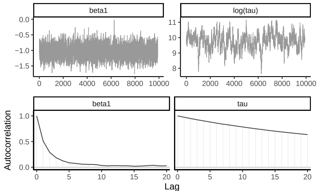
Figure 7.9: Trace plots (top) and correlograms (bottom) for two parameters of the Gibbs sampler for the Tokyo rainfall data, with block updates.
