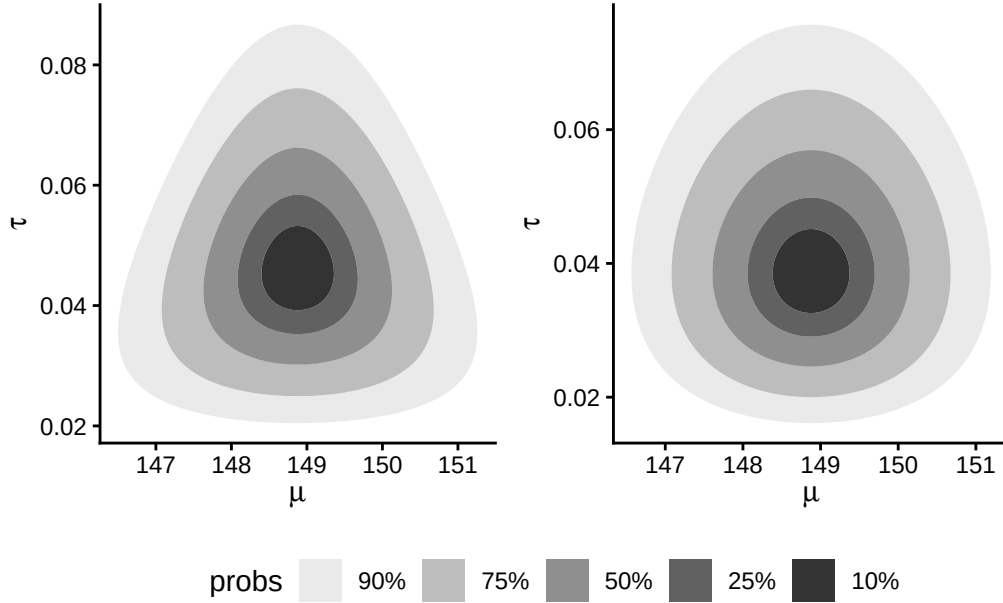
Figure 10.3: Bivariate density posterior for the conjugate Gaussian-gamma model (left) and CAVI approximation (right).
