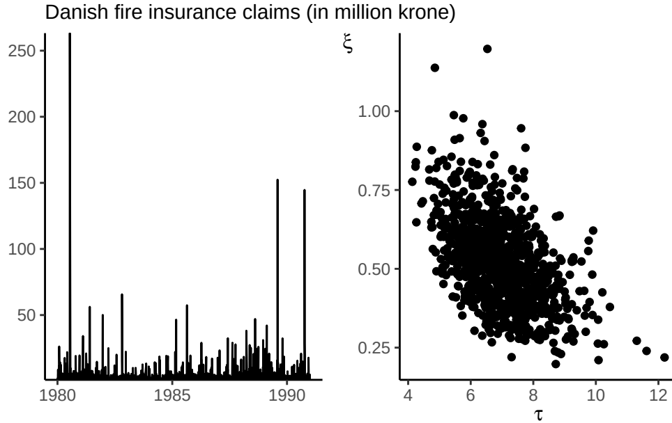
Figure 2.7: Time series of Danish fire claims exceeding a million krone (left) and posterior samples from the scale \tau and shape \xi of the generalized Pareto model fitted to exceedances above 10 million krone (right).
