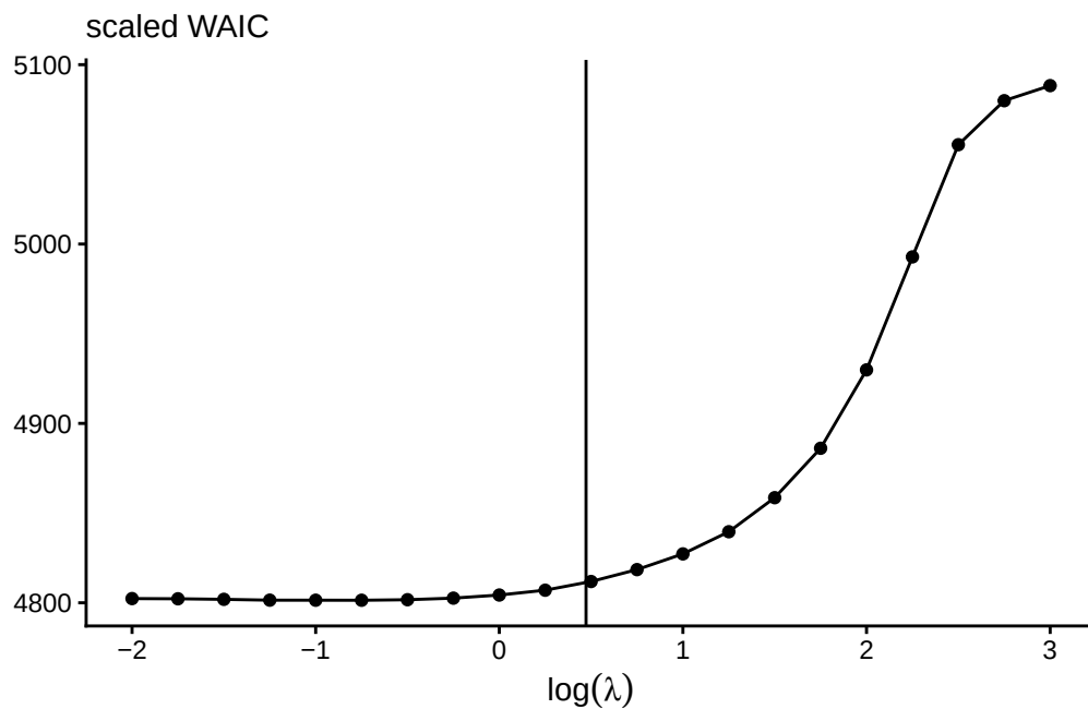
Figure 7.6: Widely applicable information criterion for the Bayesian LASSO problem fitted to the diabetes data, as a function of the penalty \lambda .
