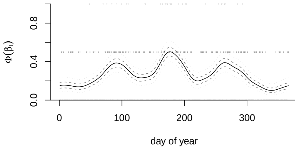
Figure 7.10: Tokyo rainfall fitted median probability with 50% and 89% pointwise credible intervals as a function of time of the year, with the proportion of days of rain (points).
