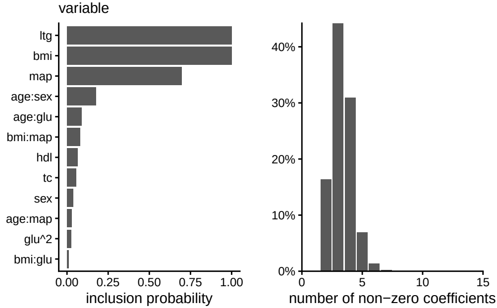
Figure 8.3: Probability of inclusion of variables (left) and posterior distribution of the number of non-zero components (right) for the discrete spike-and-slab fitted to the diabetes data, including 56 covariates with quadratic terms and interactions.
