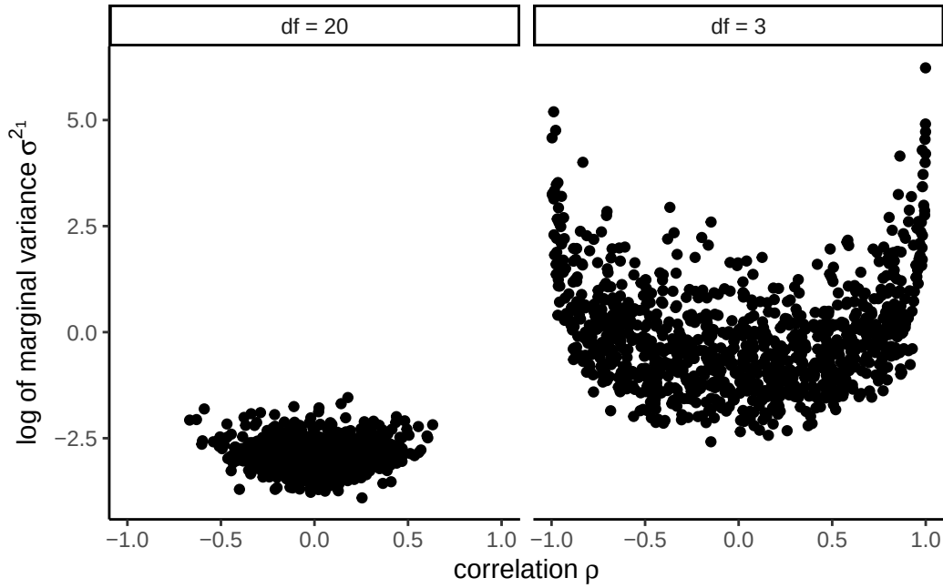
Figure 8.2: Prior draws from a bivariate inverse Wishart with identity scale matrix and \nu \in \{3, 20\} degrees of freedom.
