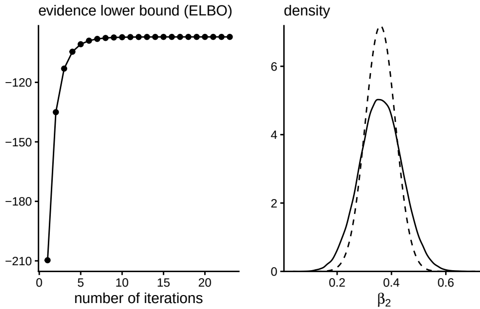
Figure 10.5: Probit regression with CAVI for the Duke and Amir (2023) data. Left: ELBO as a function of the number of iterations until convergence. Right: marginal density approximation for a regression coefficient with kernel density estimation of the true density (full line) versus variational approximation (dashed).
