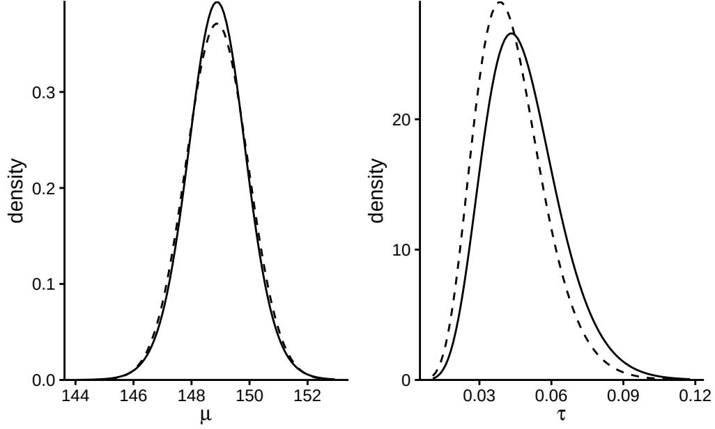
Figure 10.4: Marginal posterior density of the mean and precision of the Gaussian (full line), with CAVI approximation (dashed).
