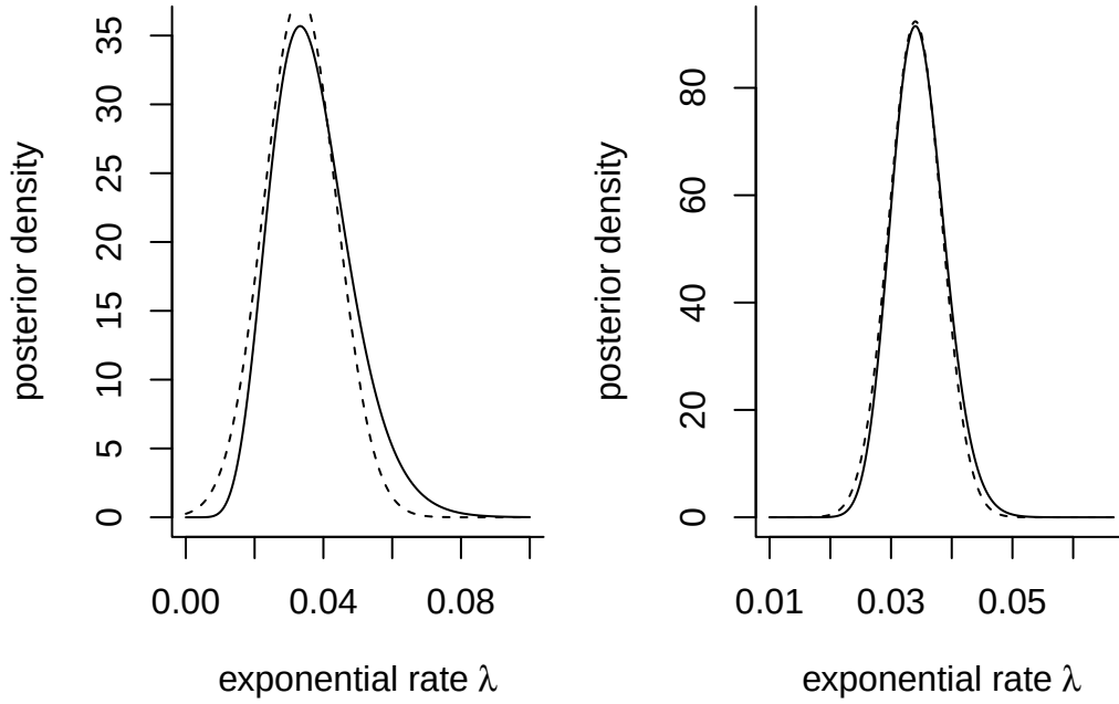
Figure 9.2: Gaussian approximation (dashed) to the posterior density (full line) of the exponential rate \lambda for the waiting dataset with an exponential likelihood and a gamma prior with a = 0.01 and b = 0.01 . The plots are based on the first 10 observations (left) and the whole sample of size n = 62 (right).
