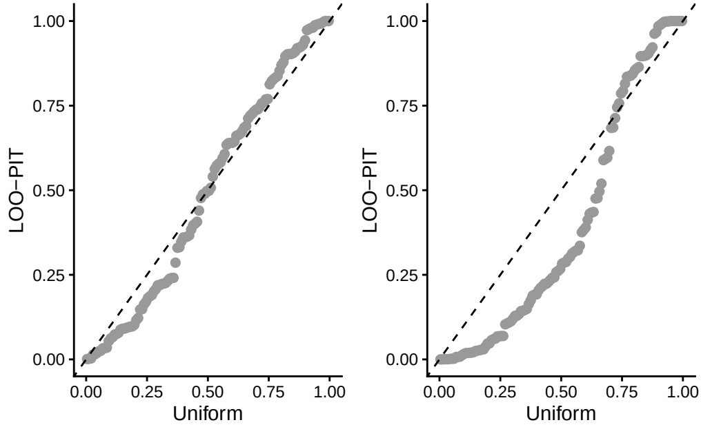
Figure 7.7: Probability-probability plots based on leave-one-out cross validation for model for the Poisson hierarchical model with the individual random effects (left) and without (right).
