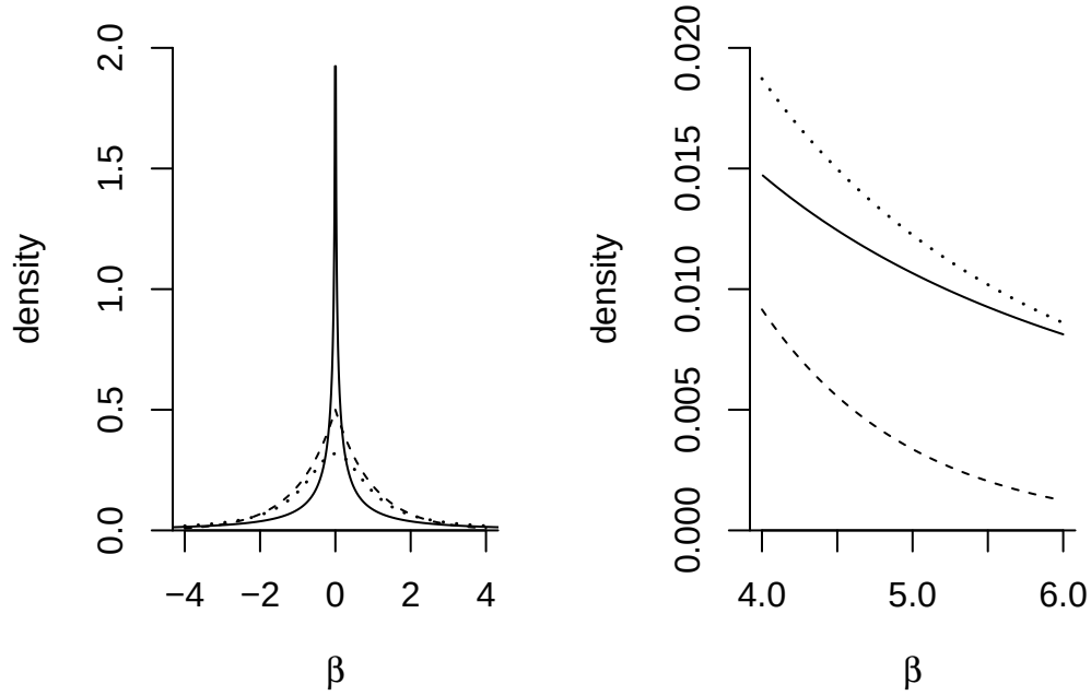
Figure 8.5: Marginal density for a regression coefficient \beta with horseshoe prior (full), Laplace (dashed) and a Student- t (thick dotted). The plot on the right shows the tail behaviour. The density of the horseshoe is unbounded at the origin. Inspired from Figure 1 of Carvalho et al. (2010).
