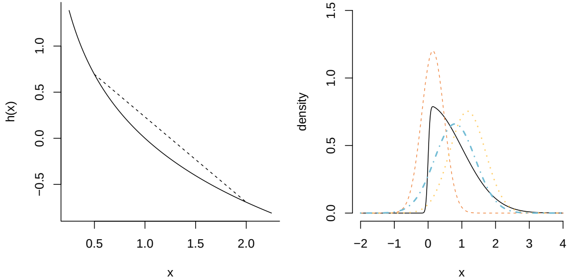
Figure 10.2: Left panel: the convex function h(x) = -\log(x) , with a straight line between any two points falls above the function. Right panel: a skewed density with the Laplace Gaussian approximation (dashed orange), the Gaussian variational approximation (reverse Kullback–Leibler divergence, dotted yellow) and the Gaussian that minimizes the Kullback–Leibler divergence (dot-dashed blue).
