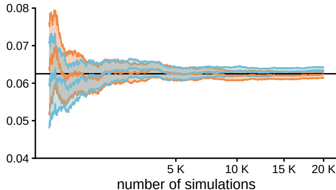
Variance estimation
