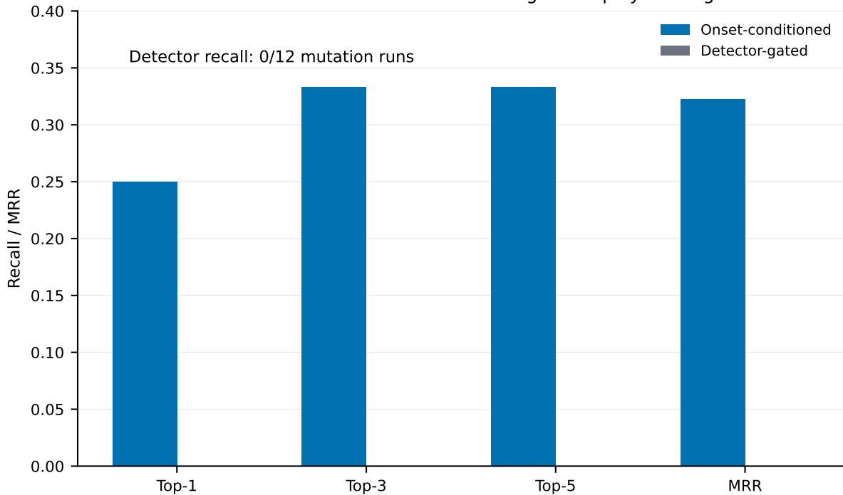
Onset-conditioned versus detector-gated replay ranking
