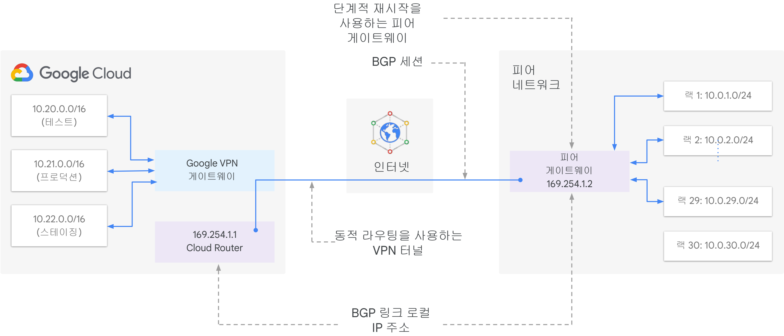
Cloud Router
