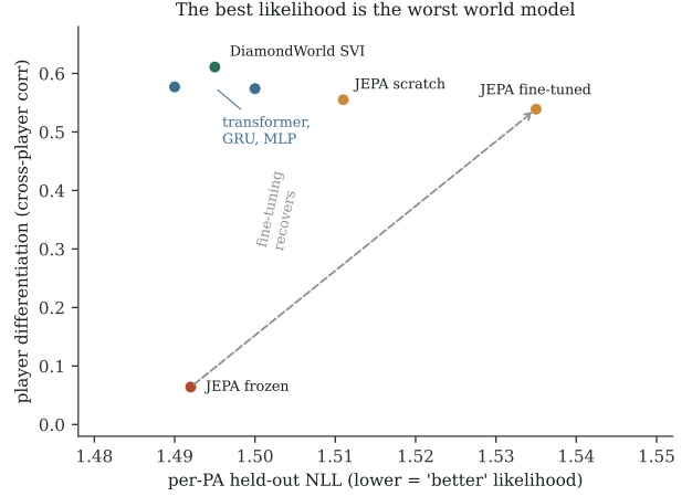
Figure 8. Held-out likelihood versus player differentiation. A frozen self-supervised probe minimizes NLL and cannot tell players apart; fine-tuning the same encoder recovers differentiation.
