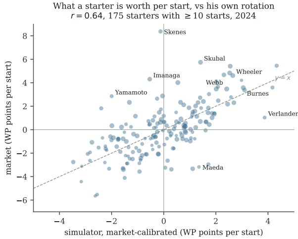
Figure 8. Win probability added per start relative to the pitcher’s own rotation, simulator (market-calibrated, x ) vs market ( y ), for 175 starters with at least ten 2024 starts. r = 0.64 ; r = 0.51 to 0.54 when the two are measured on disjoint starts.
