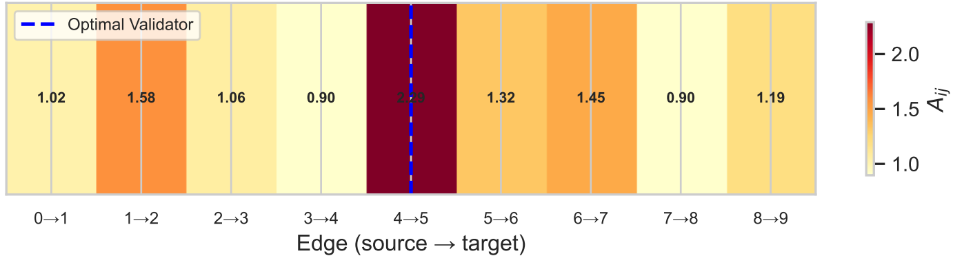
Amplification Factors A_{ij} Along Chain (m=10)
