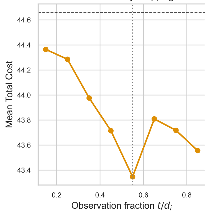
Predictive Early Stopping
