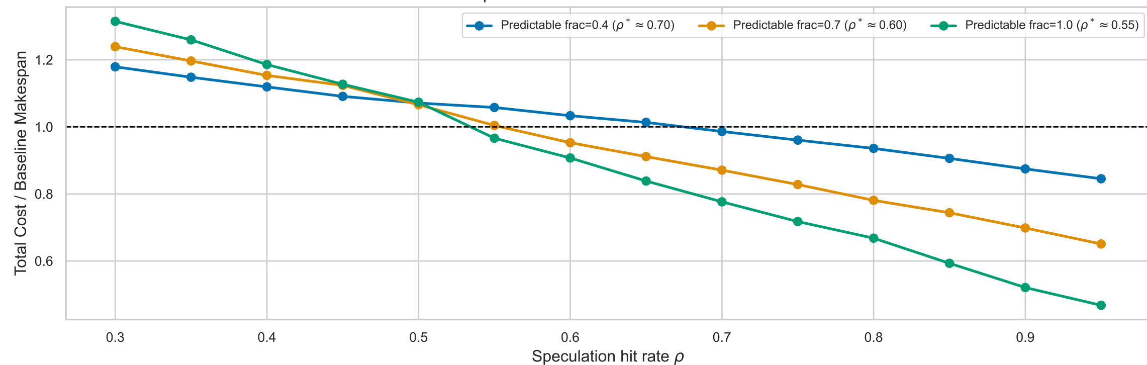
Speculative Execution on Critical Path
