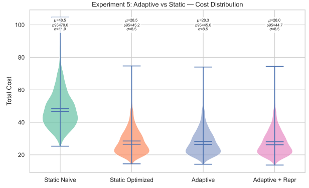
Figure 6: Experiment 5: Total cost distributions. Adaptive policies reduce both mean and tail cost.
