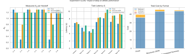
Figure 5: Experiment 4b (pilot, single run): Measured A_{ij} per handoff (left), task latency per format (center), and total cost breakdown (right) on a real 7-task Claude pipeline. Results are indicative; no confidence intervals are available from a single run.
