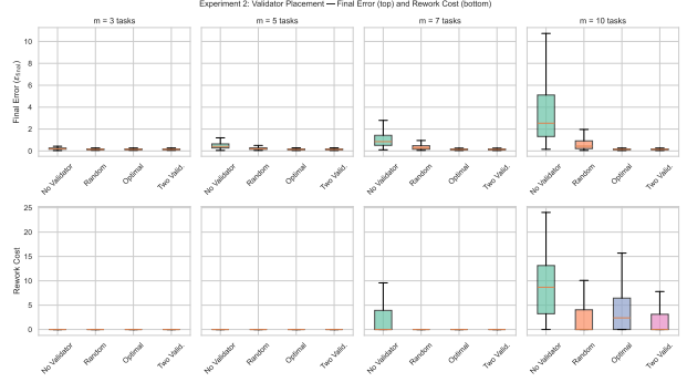
Figure 2: Experiment 2: Final error (top row) and rework cost (bottom row) by validator strategy, stratified by chain length. Optimal and two-validator conditions are identical on final error; two validators reduce rework cost by 51–80% at m \geq 7 .
