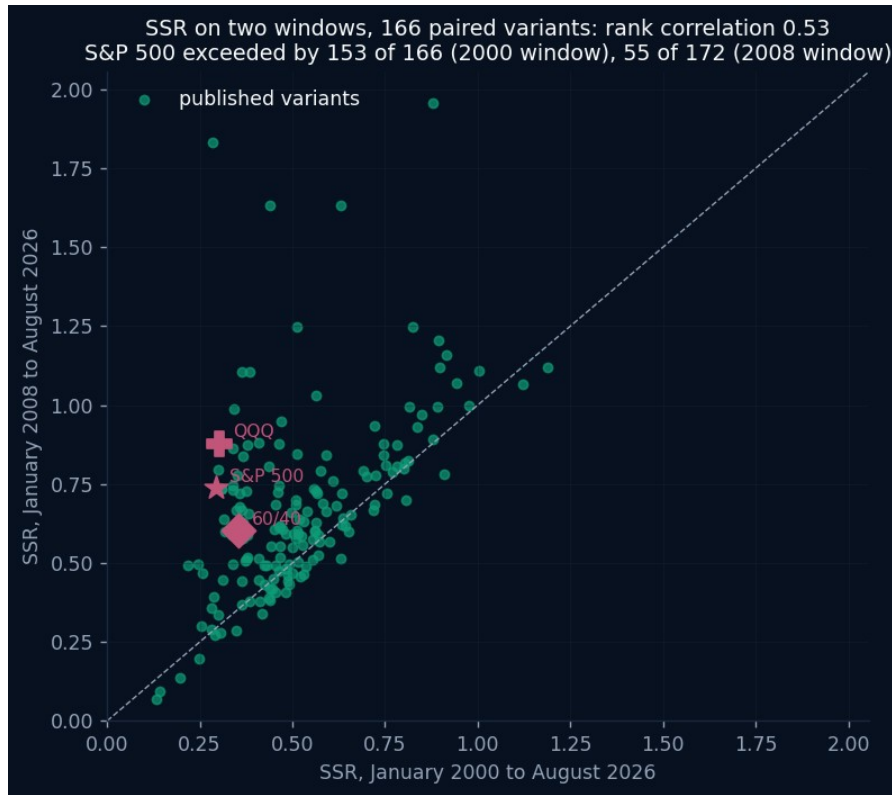
Figure 4. SSR on the January 2000 to August 2026 window against SSR on the January 2008 to August 2026 window, 166 paired variants, benchmarks marked. The counts in the title refer to the 166-variant 2000 cohort and the 172-variant 2008 cohort of Table 6.
